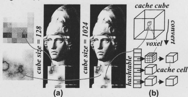
Figure 1: (a) Results of different cache cube size and (b) cache cube conception
