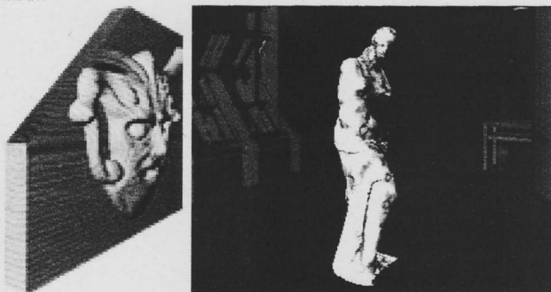
Figure 2: Rendering results.
